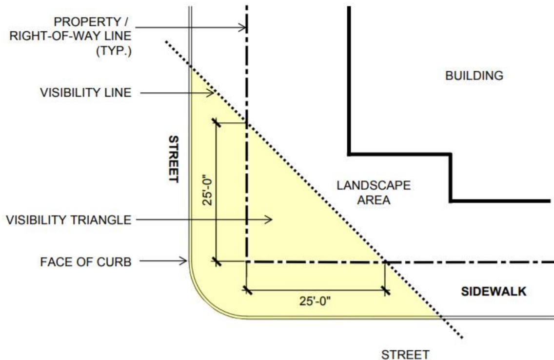
Figure 11.7.01-12: Visibility Triangle
