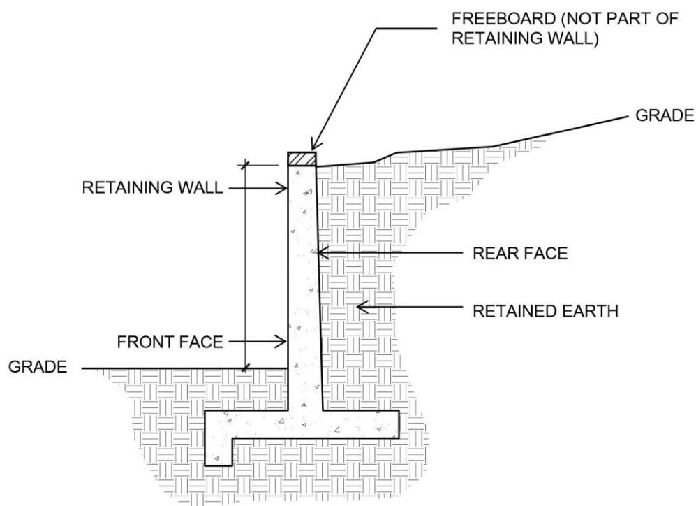
Figure 11.7.01-10: Retaining Wall—Section
