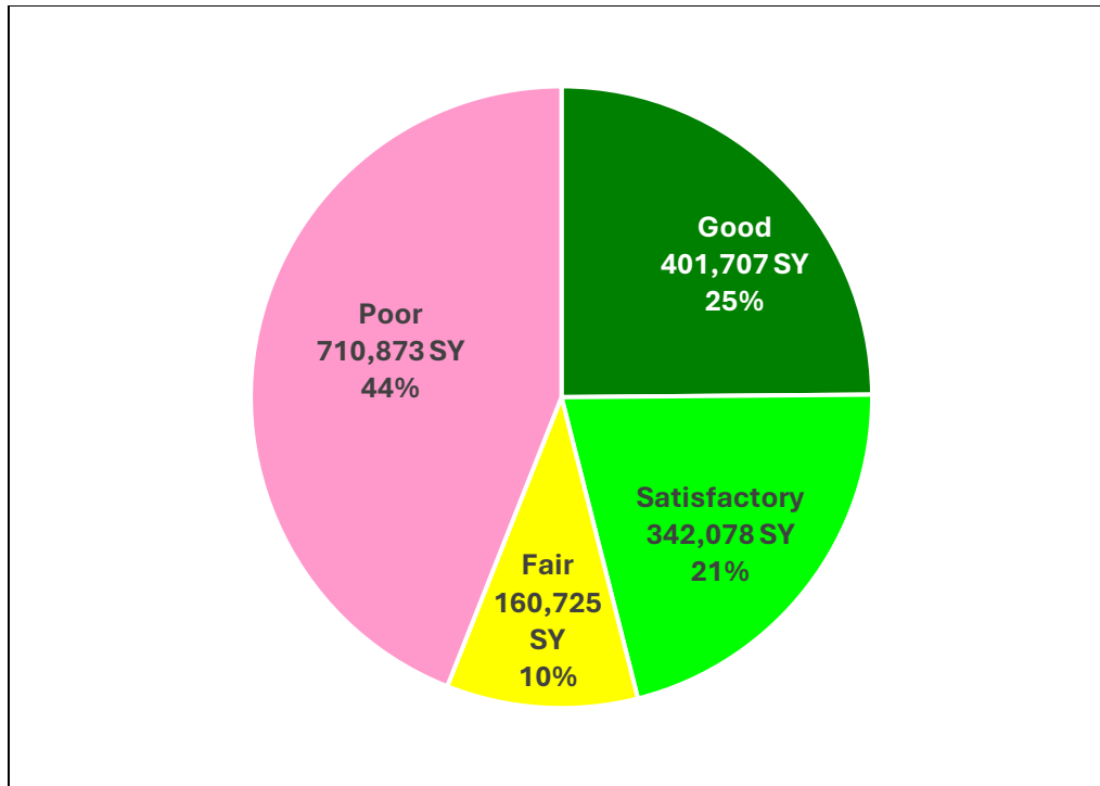
Figure 7: Pavement Condition Distribution
